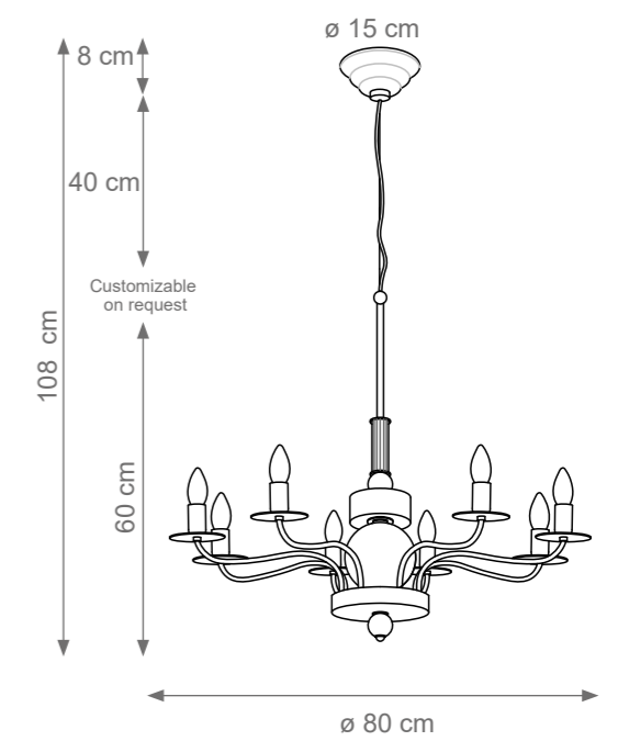
Etienne Chandelier Code: B808120 Type 8 lights electrification x Max 28W E14 CE Size: cm. 60 h x 80 ø - 5 Kg
