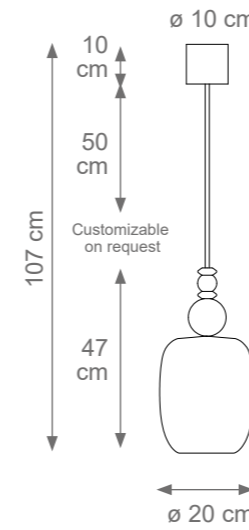
Twiggly Small Pendant Light Code: F807354 Type 1 light electrification x Max 28W E14 CE Size: cm. 47 h x 20 ø - 4 kg
