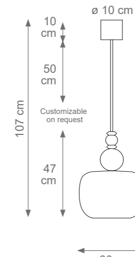
Farrah Medium Pendant Light Code: F807353 Type 1 light electrification x Max 28W E14 CE Size: cm. 47 h x 30 ø - 5 kg
