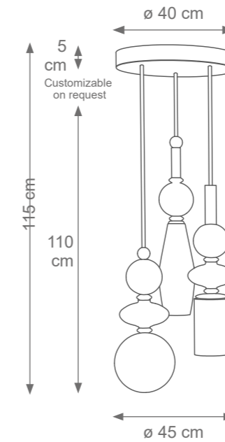
Divas Chandelier Code F807767 Type 3 lights electrification x Max 28W E14 CE Size: cm. 115 h x 45 ø - 15 kg
